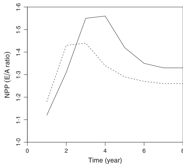
Fig. 6. Predicted time course of the NPP enhancement ratio, using the non-equilibrium version of the model. Two species with values of V_{\text{cmax}}/N yielding differing growth rates (dashed line: high A_{\text{cmax}}N = fast growth rate, solid line: low V_{\text{cmax}}/N = slow growth rate) are compared. Initially, the C a response is highest for the fast-growing species, due to a rapid leaf-area feedback. However, as the species approach equilibrium, the C a response is highest for the slow-growing species, as the leaf-area feedback is highest for this species. The relative responsiveness to C a of the two species thus depends on the time at which they are compared.
