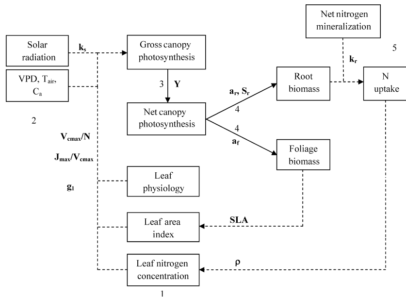
Fig. 1. Flowchart of the model used in this study, showing how species traits (abbreviations in bold; defined in Table 1) are linked. Dashed lines are the flows of information (parameters, conversion, etc.) and solid lines are flows of carbon. Numbers indicate processes as follows: (1) Scaling of leaf photosynthesis to the canopy, (2) Meteorological data as driving variables, (3) Subtraction of total respiration, (4) Annual allocation of new biomass growth to plant compartments, namely foliage and roots, and (5) Annual nitrogen uptake by the roots.
