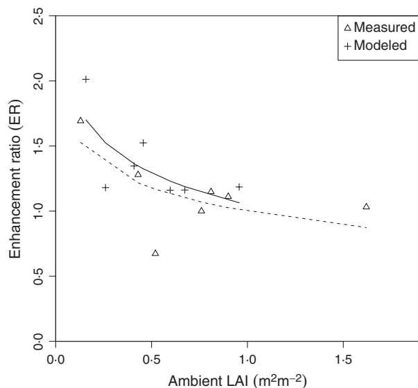
Fig. 5. Comparison of predicted NPP enhancement ratio to measurements for seven species growing in the Biodiversity, CO 2 and N free-air C a enrichment (BioCON FACE) experiment. Measured data are shown as average CO 2 enhancement ratio of NPP over the period 2003–2006 as a function of measured leaf-area index (LAI) at ambient C a . Model predictions are shown as equilibrium NPP enhancement as a function of equilibrium LAI at ambient C a . The solid curve is a best-fit regression of model output, while the dashed curve is the best-fit regression to measured data.
