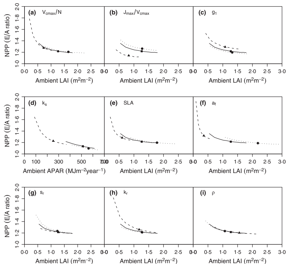
Fig. 4. Enhancement ratio of NPP, as a function of equilibrium leaf-area index (LAI) of a monoculture at ambient C_a . Each panel shows the effect of a different trait (indicated on the panel). The three curves in each panel correspond to species with three different values for that trait (base, low and high trait values). The line corresponds to the base value, the dashed line corresponds to the low value, and the dotted line corresponds to the high value. Each curve was generated by varying carbon-use efficiency ( Y ). The point on each curve indicates where Y = 0.5 . Note: the graph for the trait k_s (d) has ambient absorbed photosynthetically active radiation (APAR), rather than ambient LAI, on the x -axis (see text).
