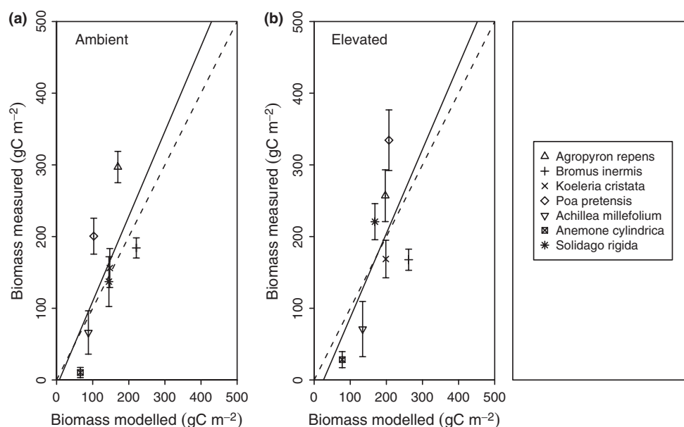
Fig. 2. Model validation against measured biomass data from the Biodiversity, CO 2 and N (BioCON) experiment. Modelled and measured total biomass of seven species (four C_3 grasses and three C_3 forbs) under ambient C_a in panel (a) or at elevated C_a in panel (b). Measured biomass data are average June biomass of species monoculture plots over the period 2003 to 2006. The modelled biomasses are the equilibrium biomass values of the model when parameterized with the species traits for the seven BioCON species (Table S1, Supporting Information). The solid line is the regression line while the dashed line is the 1 : 1 line. The R^2 values for modelled vs. measured biomass under ambient and elevated C_a are 0.45 and 0.43, respectively.
