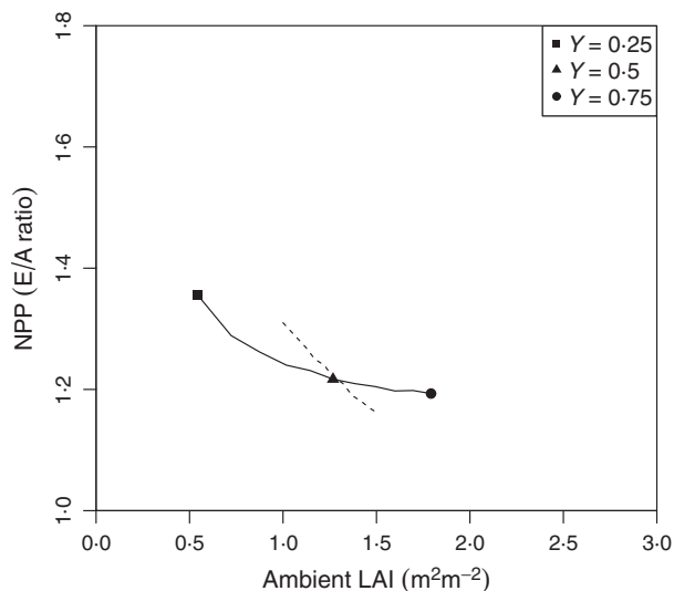
Fig. 3. Enhancement ratio of NPP (equilibrium NPP at elevated C_a divided by that at ambient C_a ) as a function of equilibrium leaf-area index (LAI) at ambient C_a , illustrating sensitivity to respiration rates using both respiration assumptions. The solid curve is generated by varying the carbon-use efficiency ( Y ) from its baseline value (0.5) by \pm 50\% . The highest NPP enhancement ratio and lowest ambient LAI are obtained for the lowest Y . The dashed curve is obtained by varying species respiration rates ( R_f , R_r ) by \pm 50\% . Similarly, the highest C_a responsiveness and lowest ambient LAI are obtained for the highest respiration rates.
